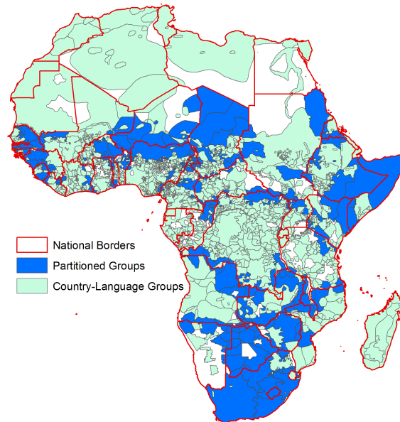
Figure 3: Language Partitions
